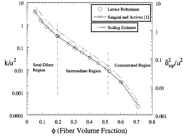
FIG. 5. Hydraulic permeability: two-dimensional square array of periodic cylinders. Nondimensional hydraulic permeabilities calculated using the LB method are compared with the result of Sangani and Acrivos [1], and the scaling estimate given in Eq. (11) for a complete range of fiber volume fractions \phi . The line through their data is provided to guide the eye. The cylinder radii in the LB simulations range from 6 to 12 lattice units depending on \phi . The dashed vertical lines separate regions of transitional behavior in the hydraulic permeability. These regions include three distinct ranges of \phi , i.e., the dilute to semidilute limit, the intermediate range, and the concentrated range. The transitions between these regions occur at \phi \approx 0.2 and \phi \approx 0.52 , respectively.
