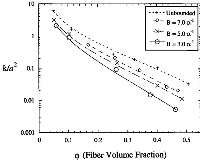
FIG. 10. Hydraulic permeability: bounded three-dimensional, disordered array of cylinders. Hydraulic permeabilities calculated using the LB method for bounded, disordered arrays of cylinders are compared with the unbounded results for the same system presented in Sec. IV. The wall to midplane separations B considered are 3, 5, and 7 Brinkman screening lengths. Hydraulic permeabilities are made dimensionless with the cylinder radius squared. The lines through the data are from a curve fitting using Eq. (14). The curve-fit parameters are given in Table III.
